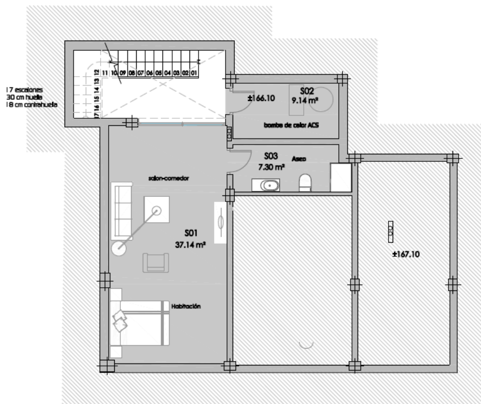
SOTANO / BASEMENT
